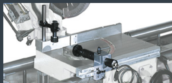
Frontal clamps (standard for CE version): for a better holding of the pieces during the cut.
