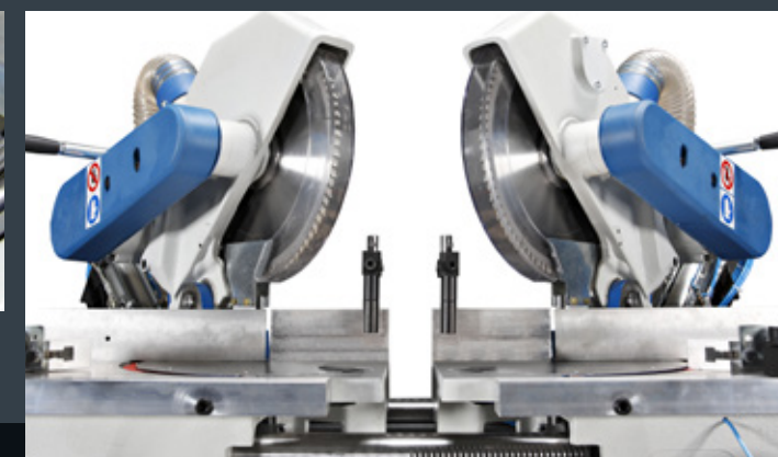
Pneumatic carriage between the two heads for the automatic shifting of the work piece when cutting short pieces. (TR2B I INT)
